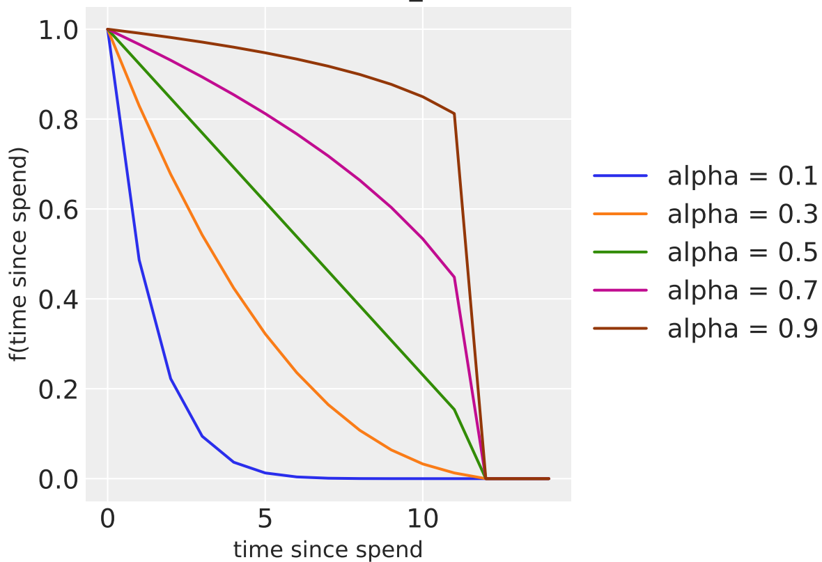
Binomial Adstock with I_{\max} = 12
